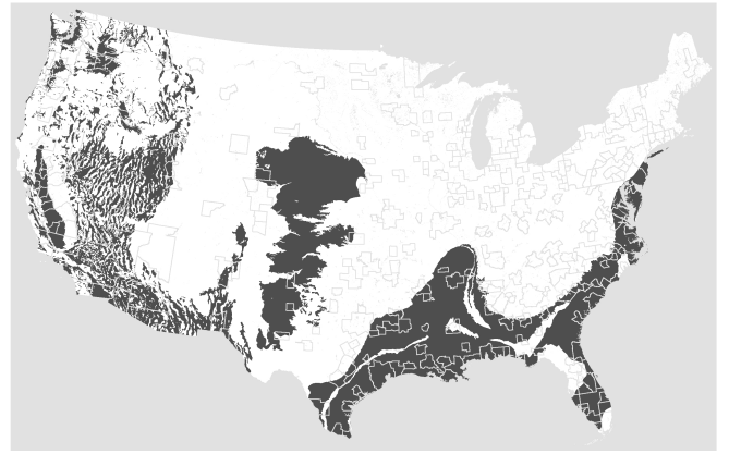
(b) Aquifers
